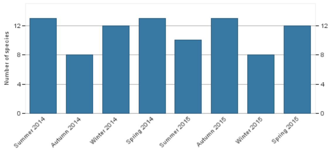
Number of bird species observed - Site 30081 Lake Yando North Rd
